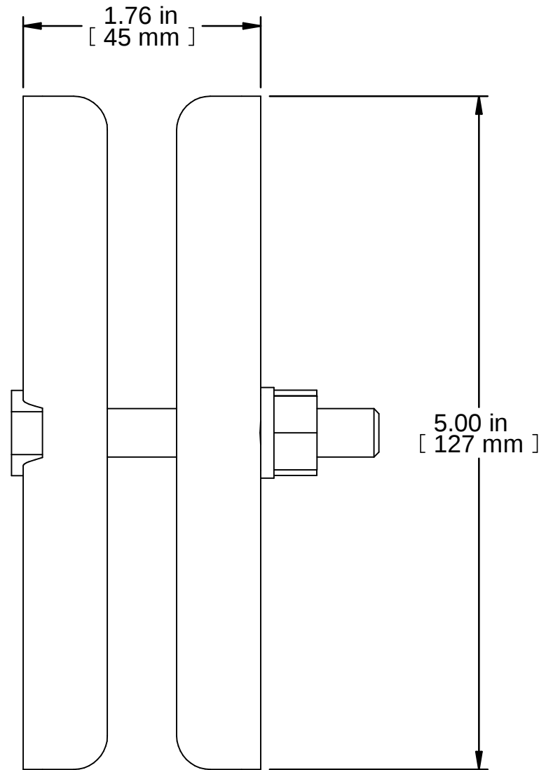
FRONT VIEW
