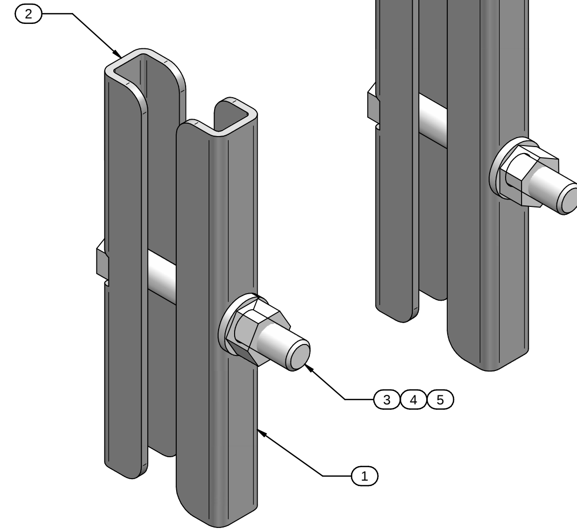
ISOMETRIC
