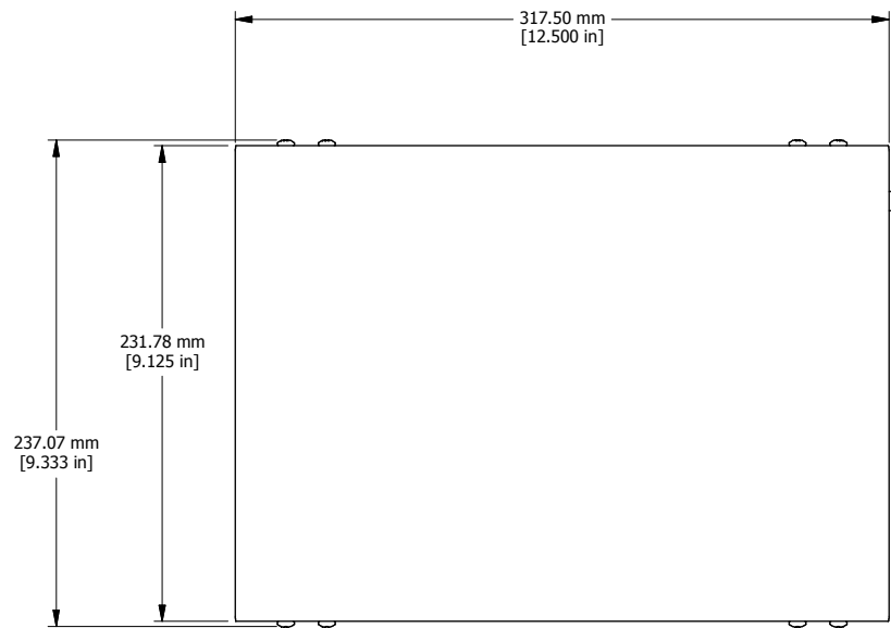
ASSEMBLY - TOP VIEW
