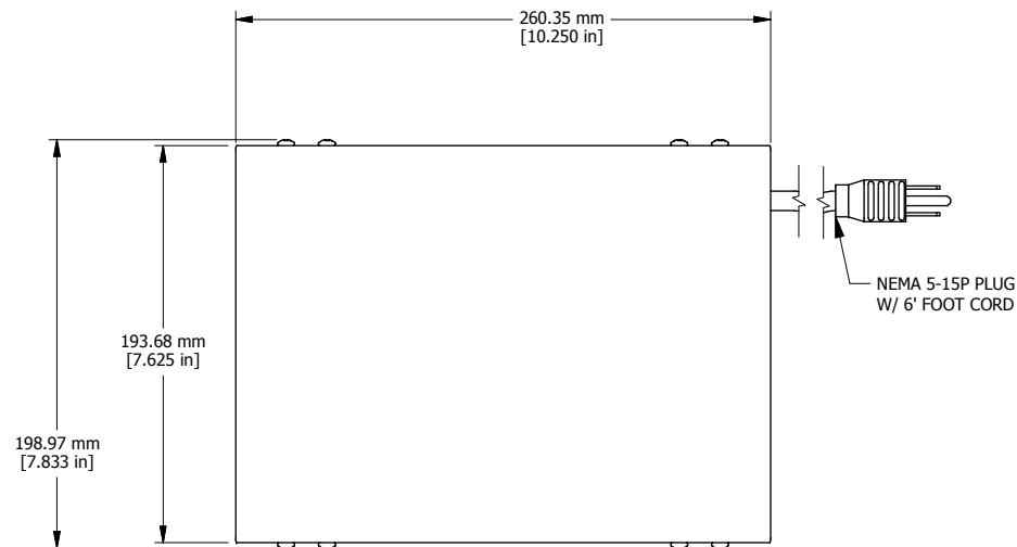
ASSEMBLY - TOP VIEW
