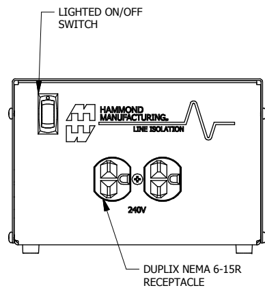
ASSEMBLY - FRONT VIEW
