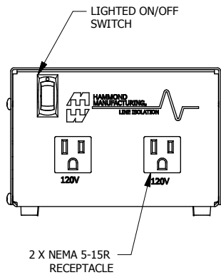
ASSEMBLY - FRONT VIEW
