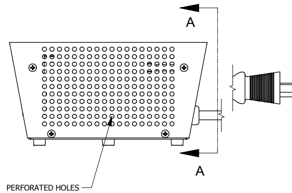
ASSEMBLY - SIDE VIEW
