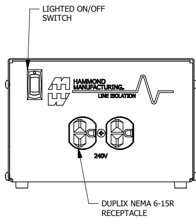
ASSEMBLY - FRONT VIEW
