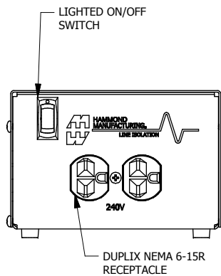
ASSEMBLY - FRONT VIEW
