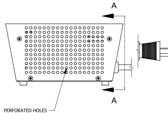
ASSEMBLY - SIDE VIEW
