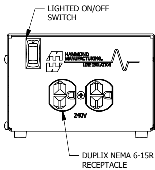
ASSEMBLY - FRONT VIEW
