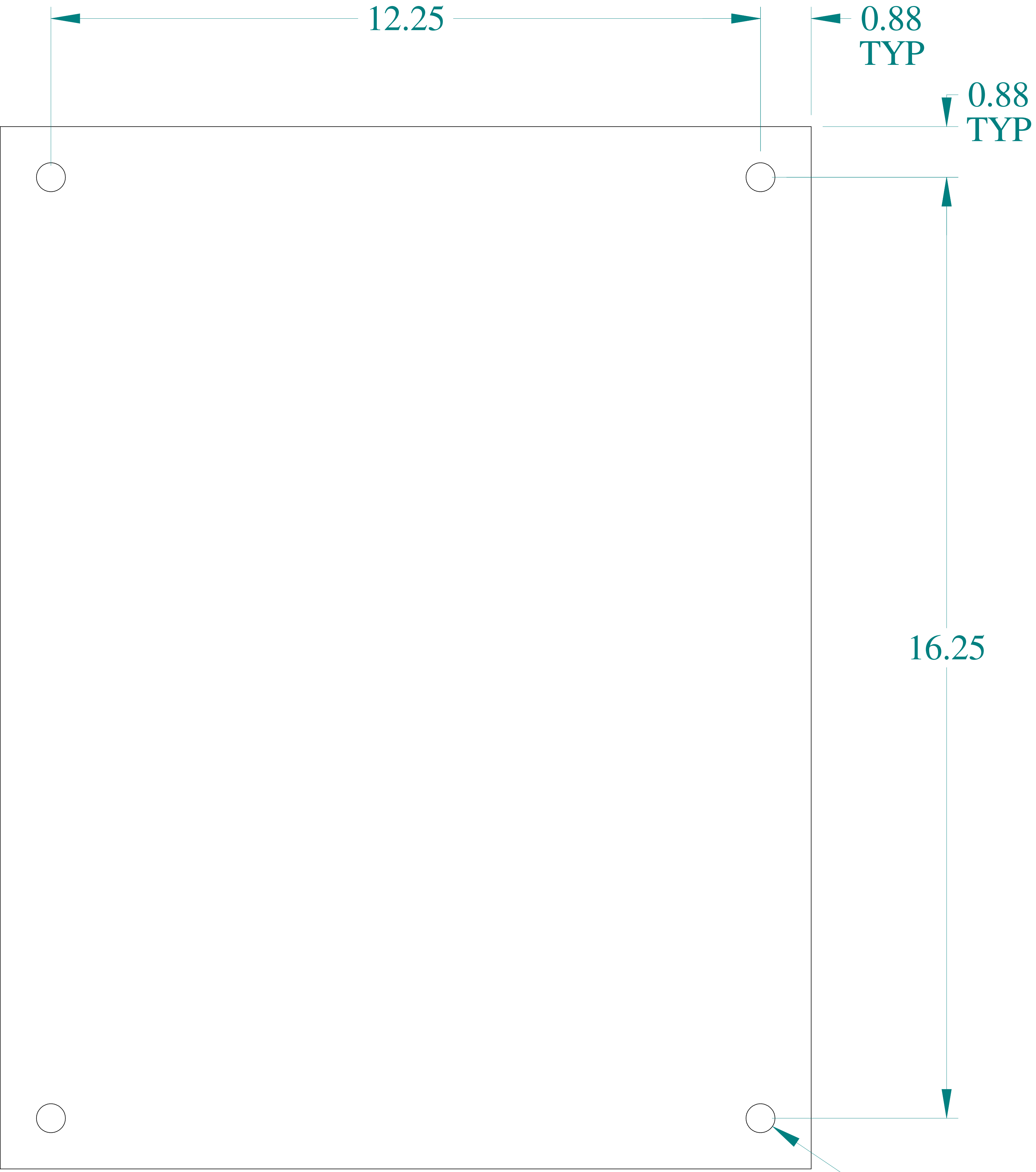
FRONT VIEW
