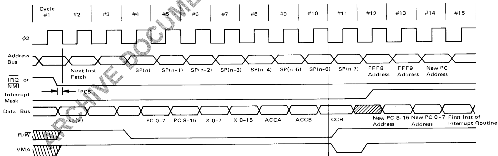
FIGURE 9 — INTERRUPT TIMING
