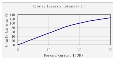
光强与正向电流曲线图 Light intensity and forward current curves
