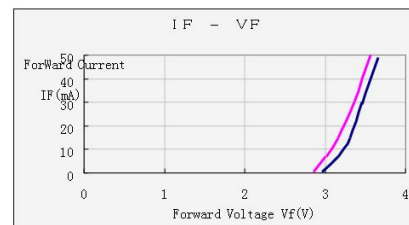
反向电流与正向电压曲线图 Reverse current vs. forward voltage plot
