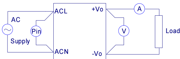
Figure 1. CBM70S Series Test Setup
