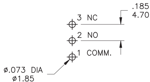
P.C.MOUNTING
