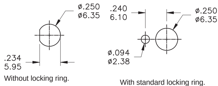
PANEL MOUNTING
