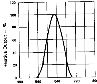
Fig. 2 SPECTRAL RESPONSE.
