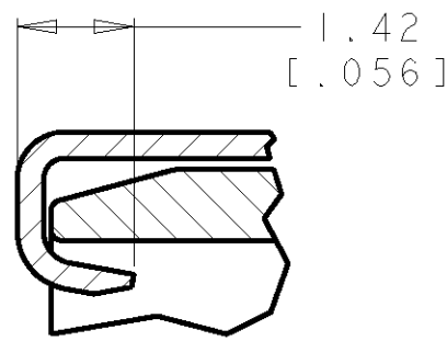
SECTION Z-Z SCALE 10:1
