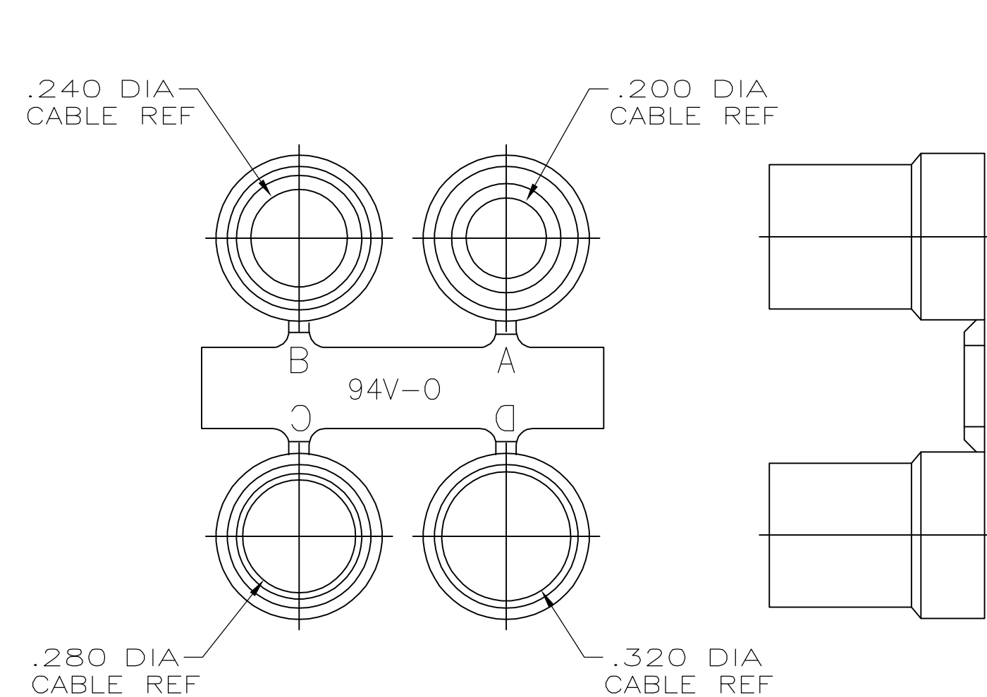
GROMMET ASSORTMENT FOR SIZES 1 & 2 ONLY
