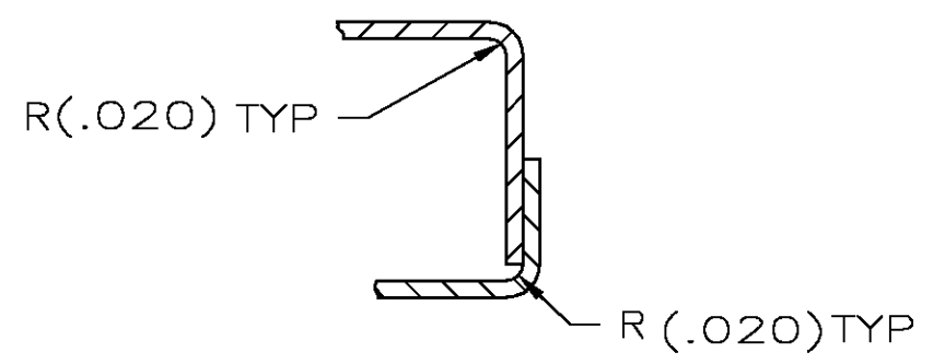
SECTION E-E SCALE 4:1
