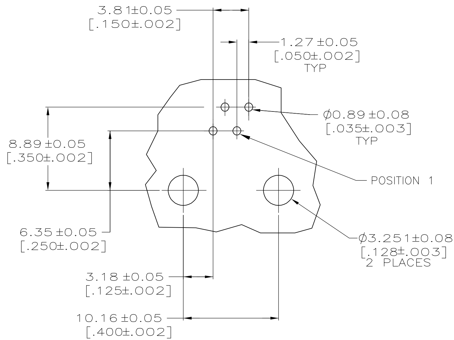
PRINTED CIRCUIT BOARD LAYOUT COMPONENT SIDE SHOWN
