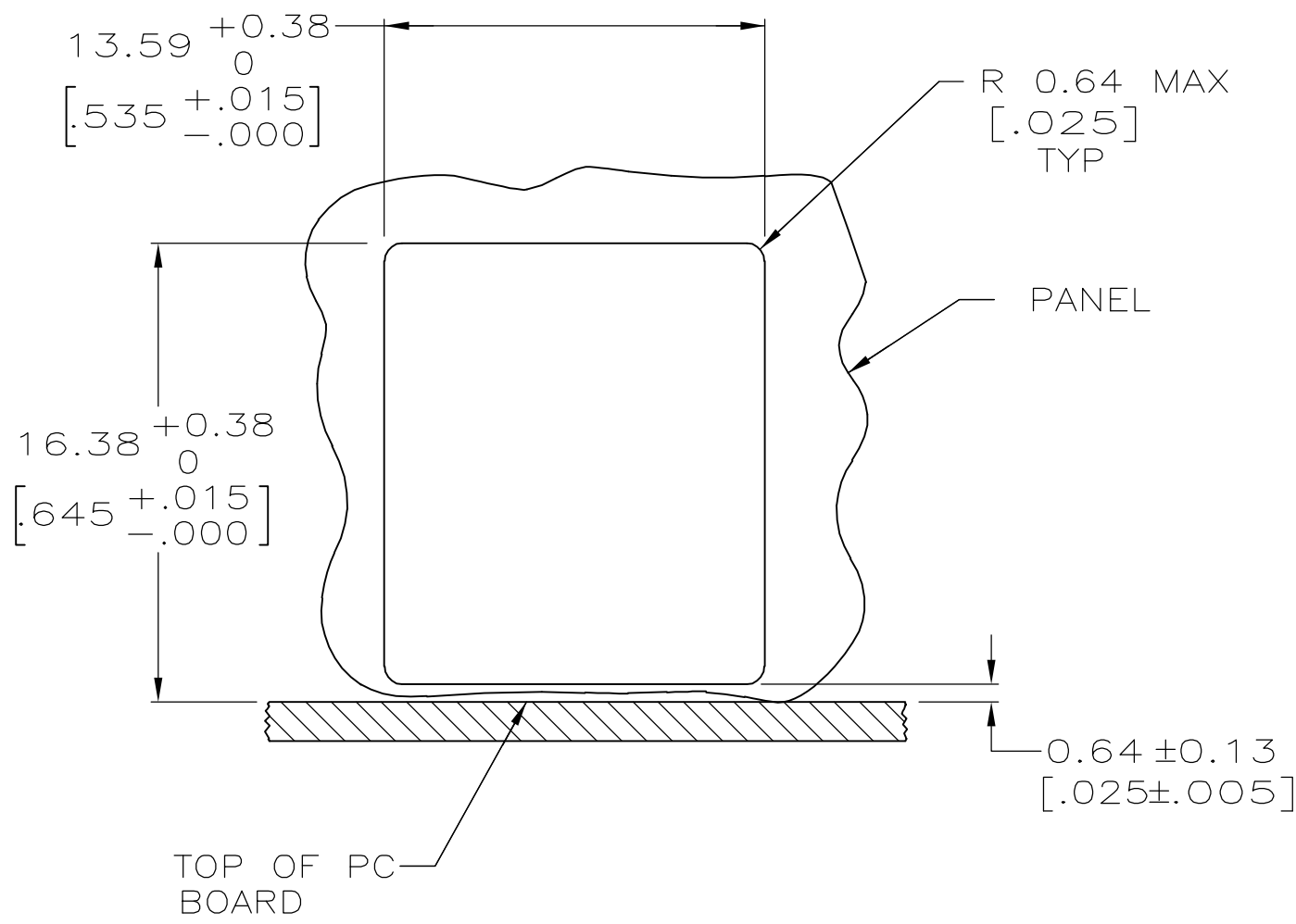
PANEL CUTOUT
