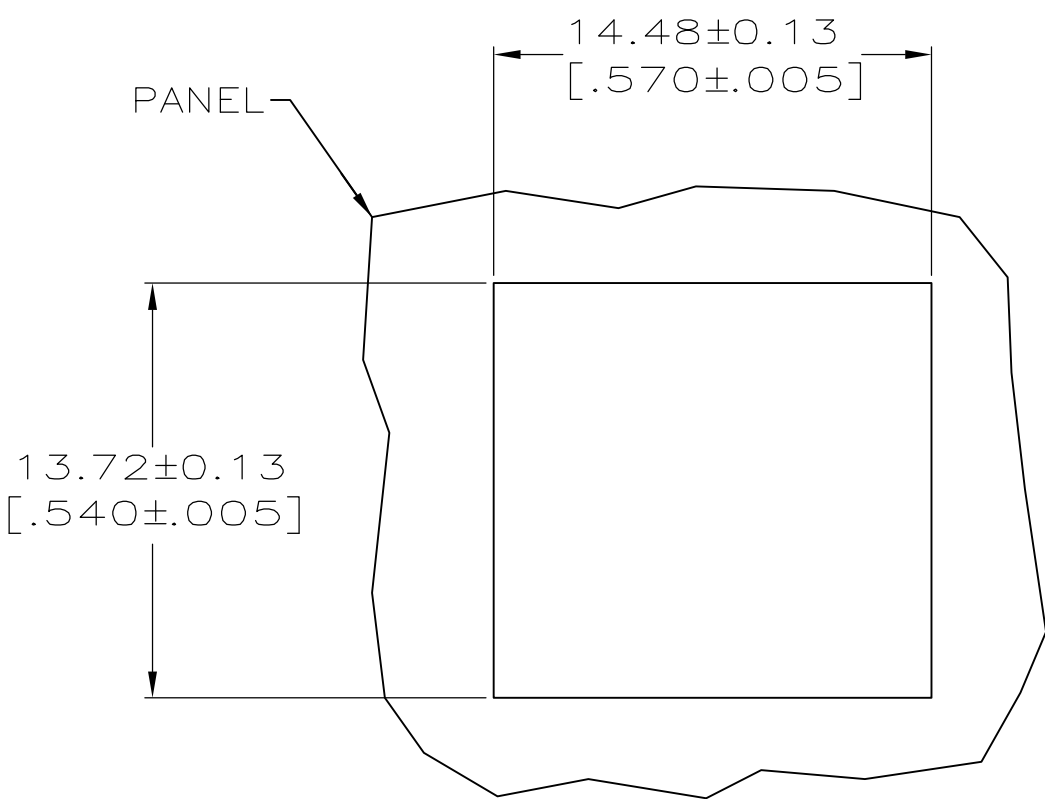
PANEL CUTOUT
