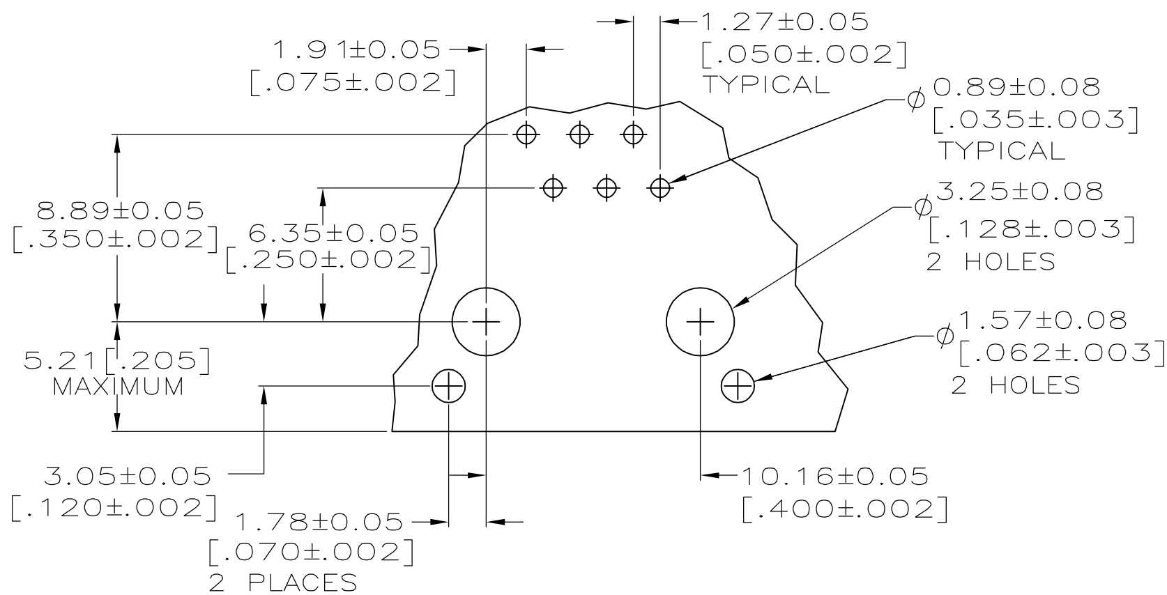
SUGGESTED PRINTED CIRCUIT BOARD LAYOUT COMPONENT SIDE
