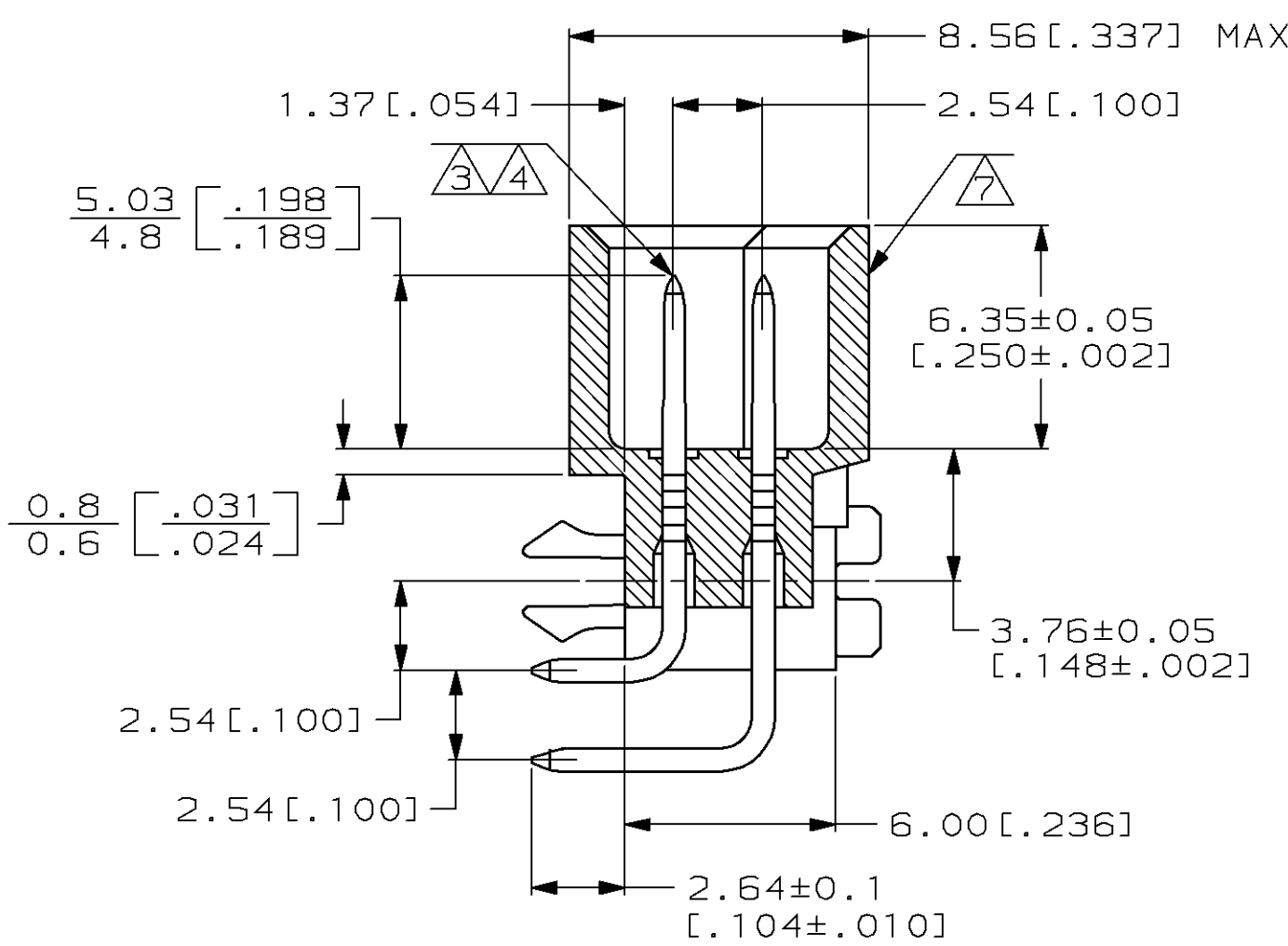
SECTION Z-Z
