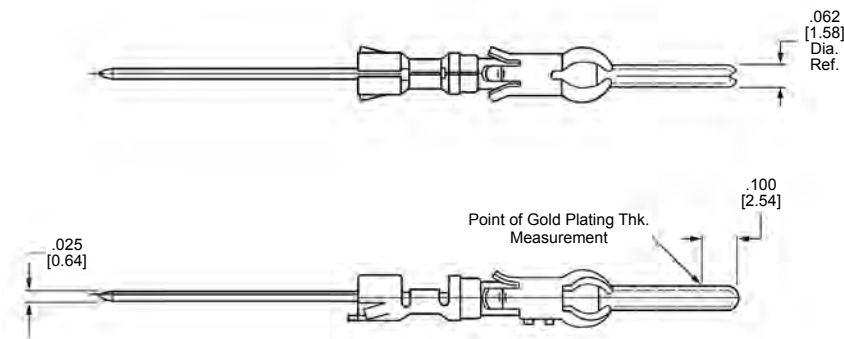
Pin
