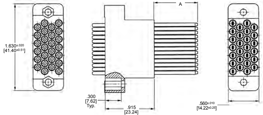
Plug Assembly
