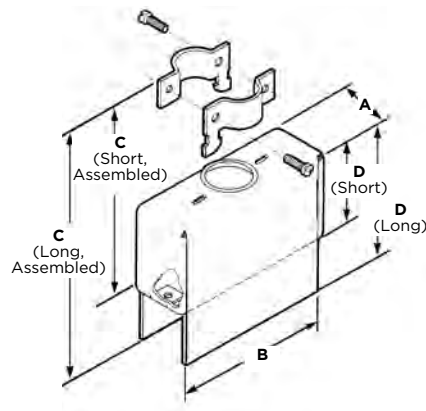
180° Cable Exit
