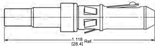
Pin
