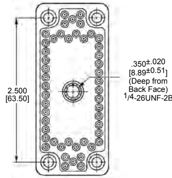
Receptacle Housing
