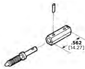
Short-Short Turnable Jackscrew, Male Part No. 203535-2 (2 Req'd.)
