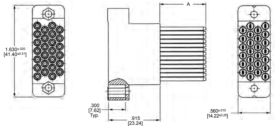
Receptacle Assembly
