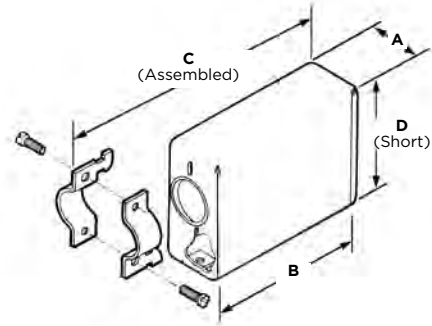
90° Cable Exit
