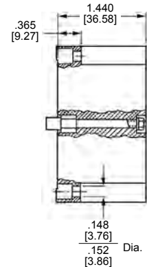
Receptacle Housing
