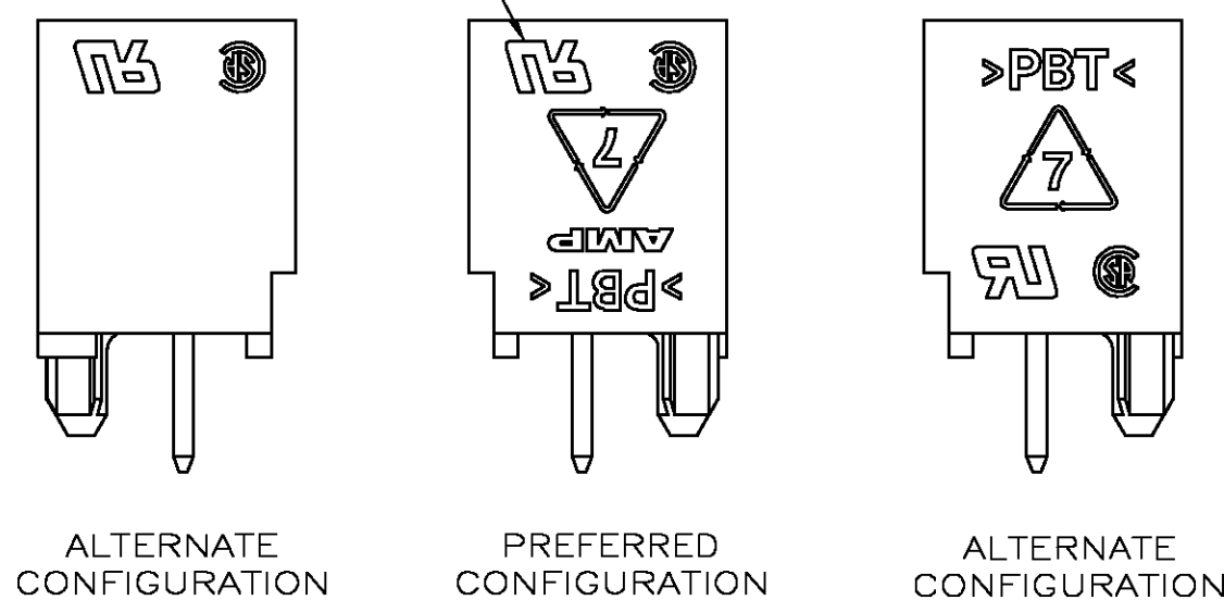
POSSIBLE MARKING CONFIGURATIONS SCALE 5:1
