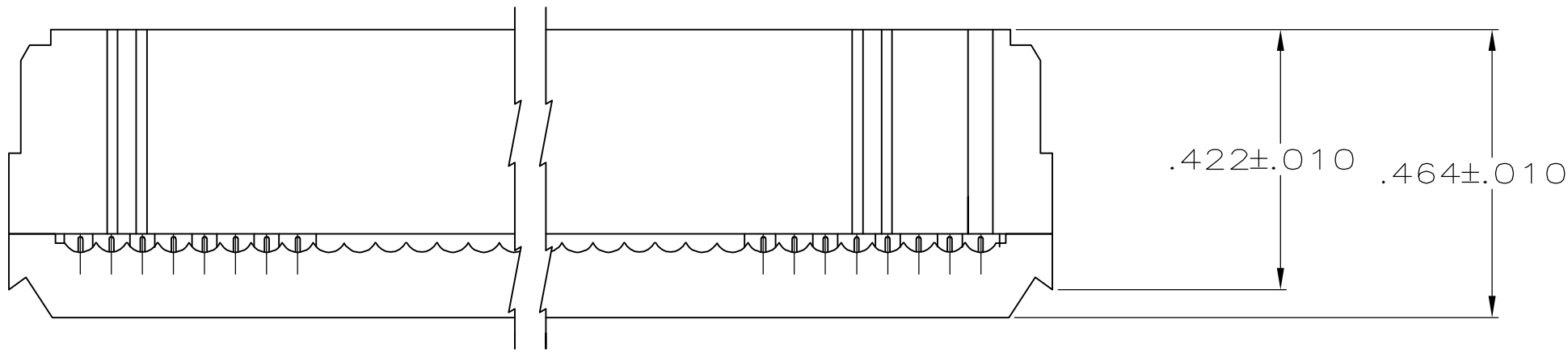
TERMINATED VIEW
