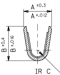
SECT. G-G
