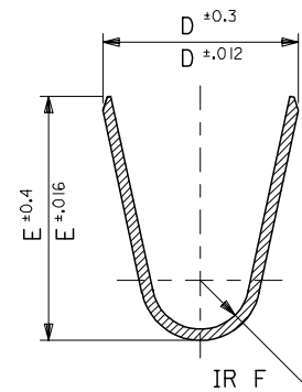
SECT. H-H
