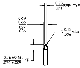
DETAIL X SCALE 5:1
