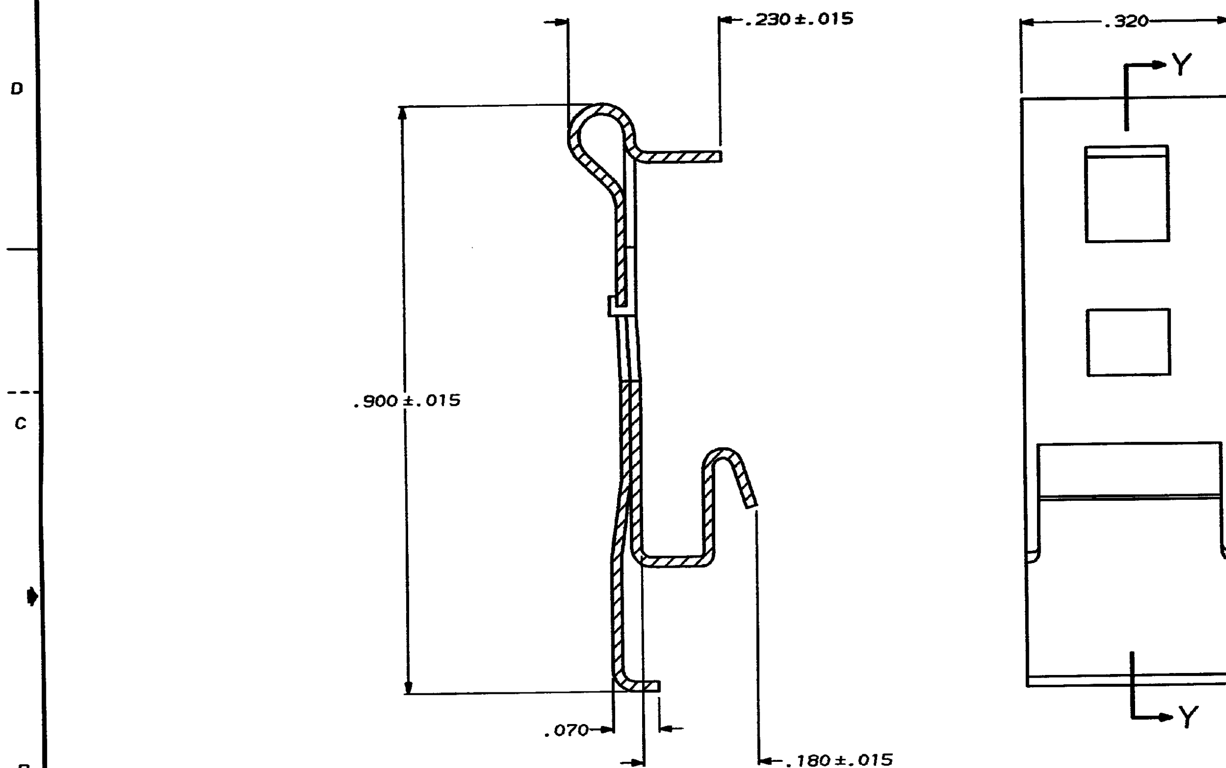
SECTION Y-Y
