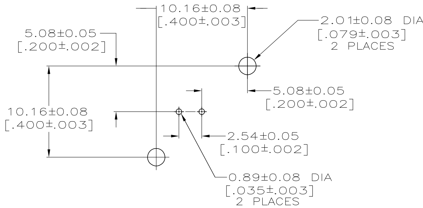
PCB CONFIGURATION
