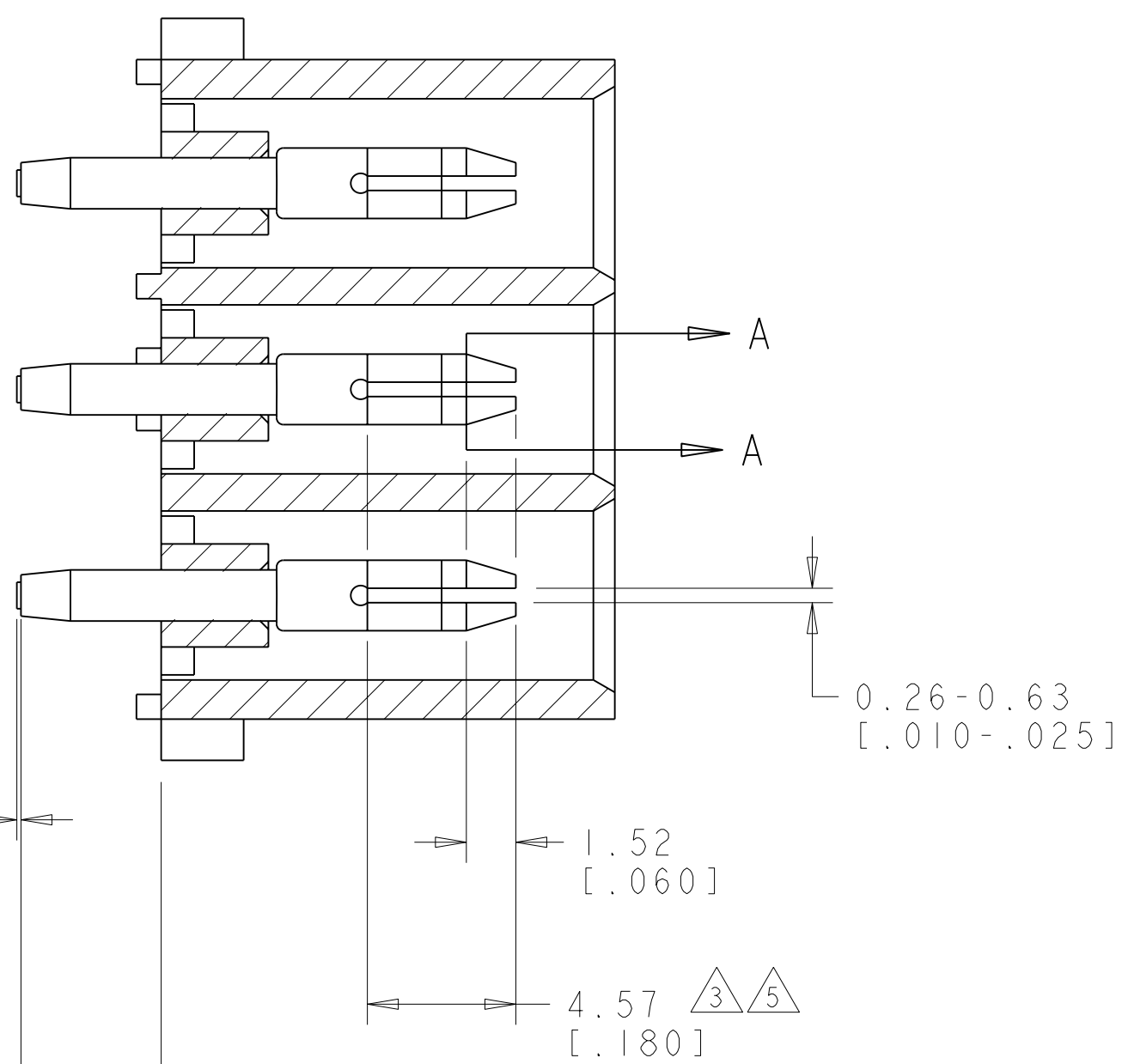
SECTION B-B
