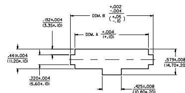
RECOMMENDED PANEL CUT-OUT DETAIL (PANEL THICKNESS .071 (1.80) MAX.)
