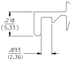
DETAIL 3 .093/(2.36) STANDARD MOUNTING EAR (SCALE 4:1)
