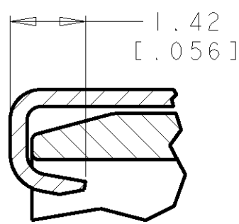
SECTION Z-Z SCALE 10:1
