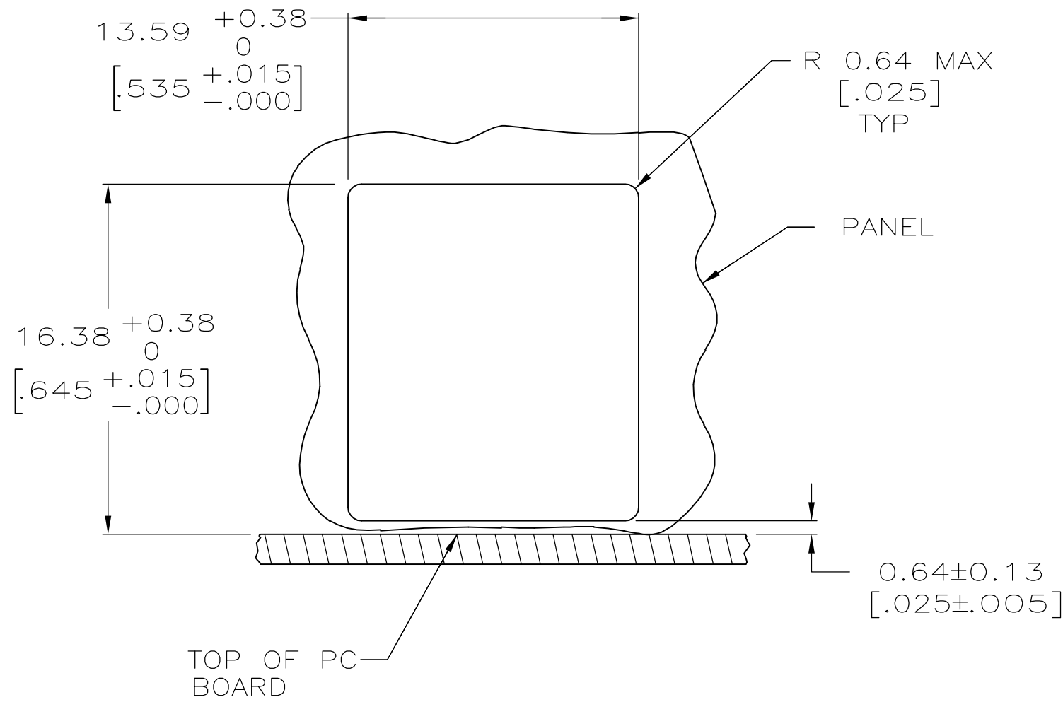
PANEL CUTOUT
