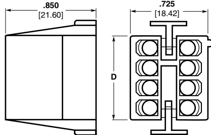
Socket Housing (Plug)
