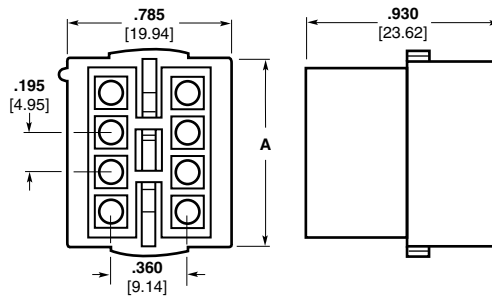
Pin Housing (Cap)
