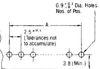
PC Board Layout (Applicable board thickness : 1.6mm)
