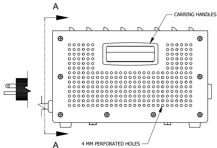
ASSEMBLY - VIEW FROM SIDE
