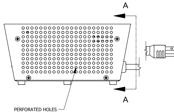
ASSEMBLY - SIDE VIEW
