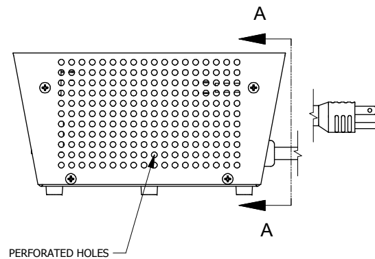
ASSEMBLY - SIDE VIEW
