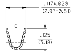
SECT. "B-B"
