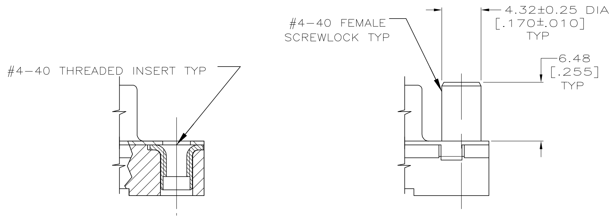
DETAIL D
