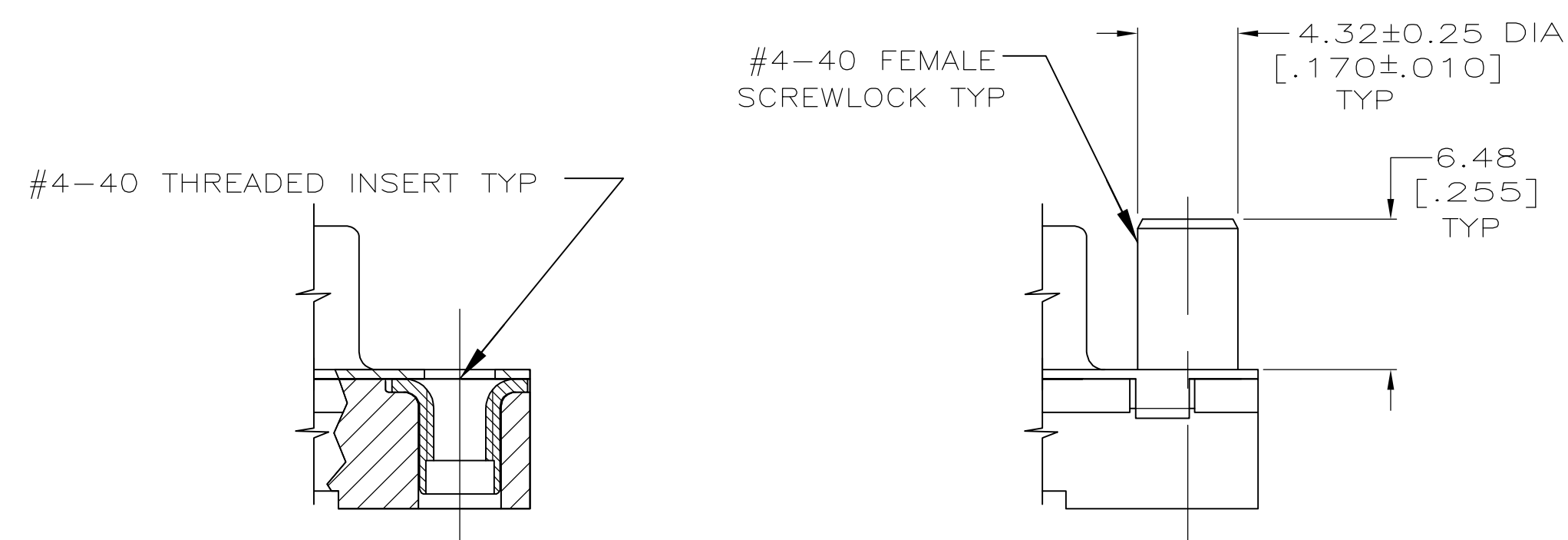
DETAIL E
