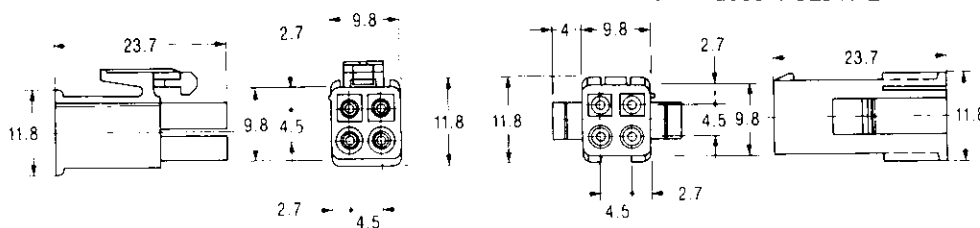
Plug (Reinforced Type)
