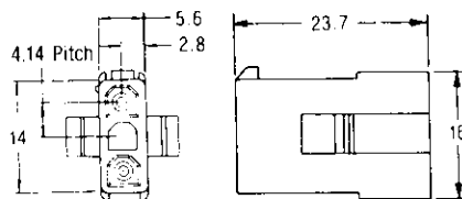
Cap (Panel Mount)
