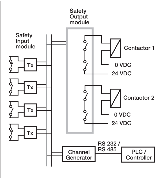
DuplineSafe Principle Diagram
