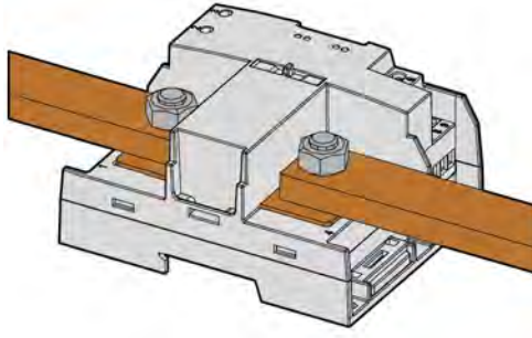
Fig. 1 Bar-bar mounting
