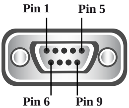
RS422/485 Pinout (9 Pin)
