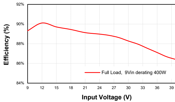
CHB500W-24S54 Eff Vs Io @25 Deg. C
