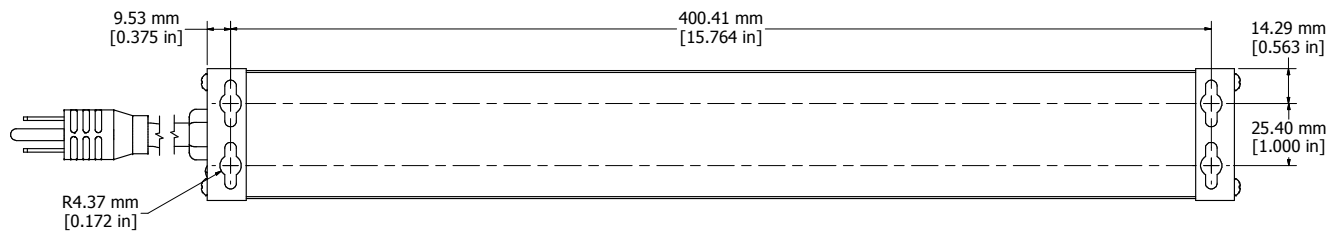
ASSEMBLY - VIEW FROM BOTTOM
