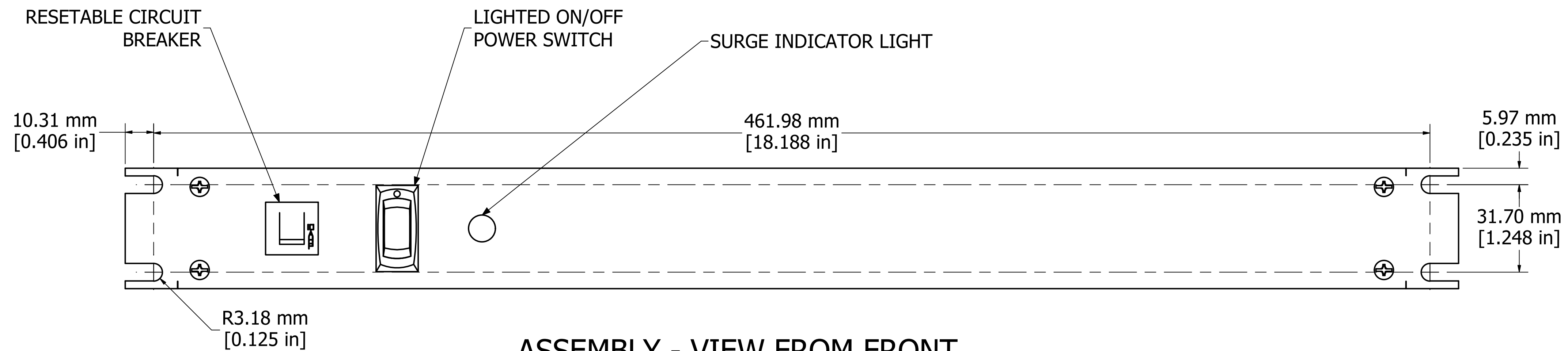
ASSEMBLY - VIEW FROM FRONT
