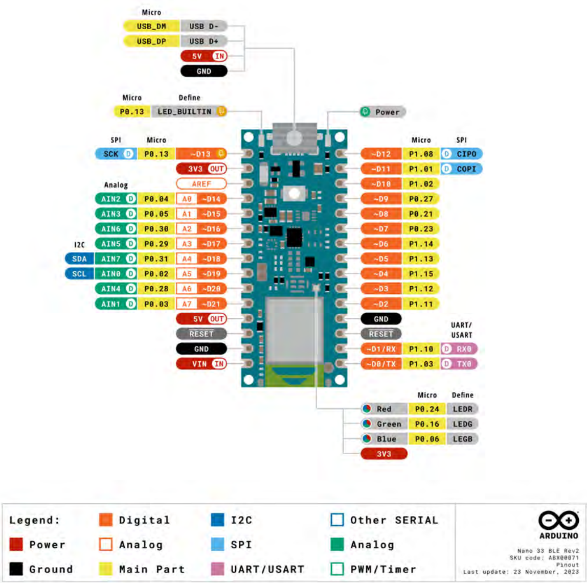
Pinout
