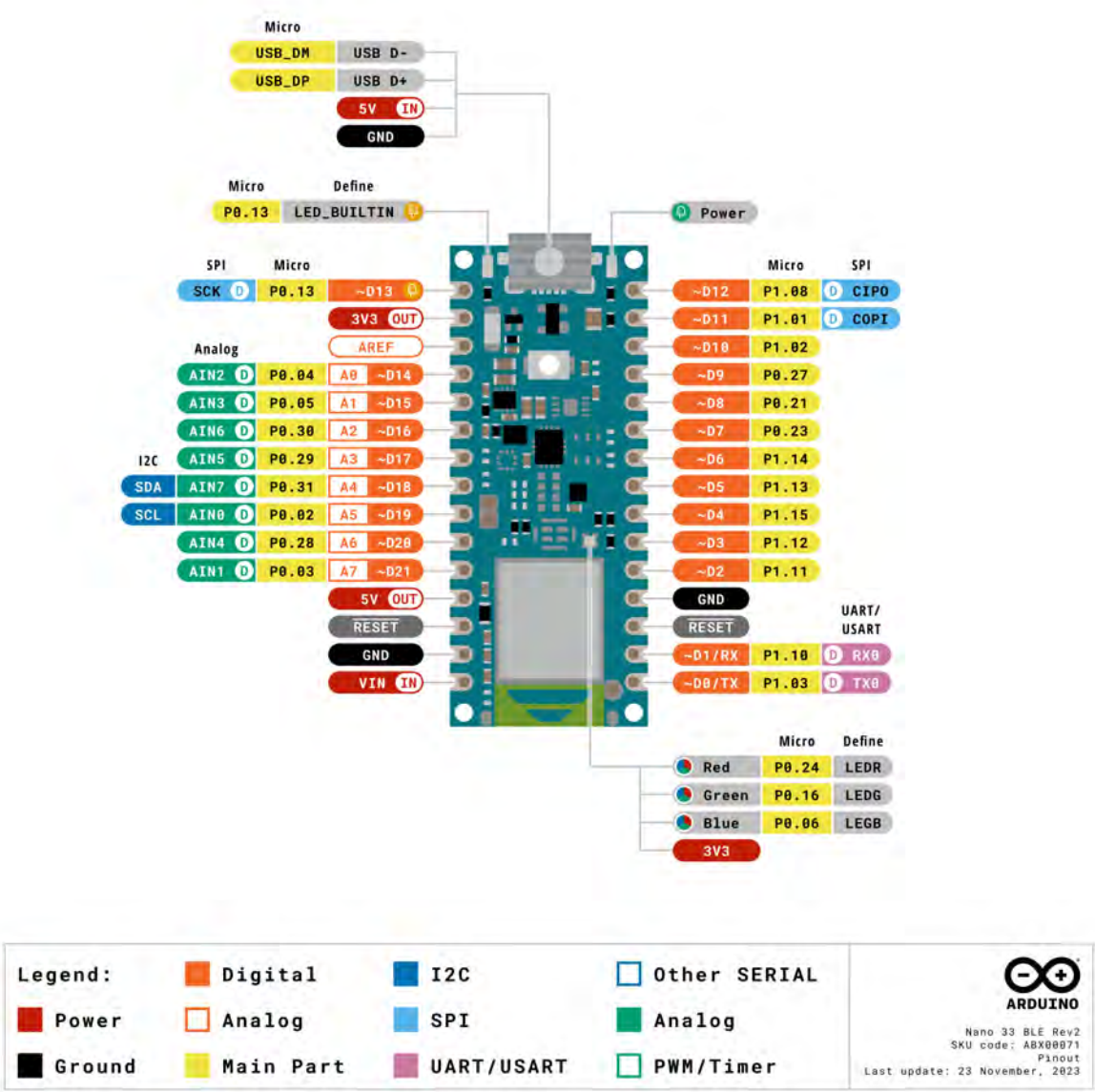
Pinout
