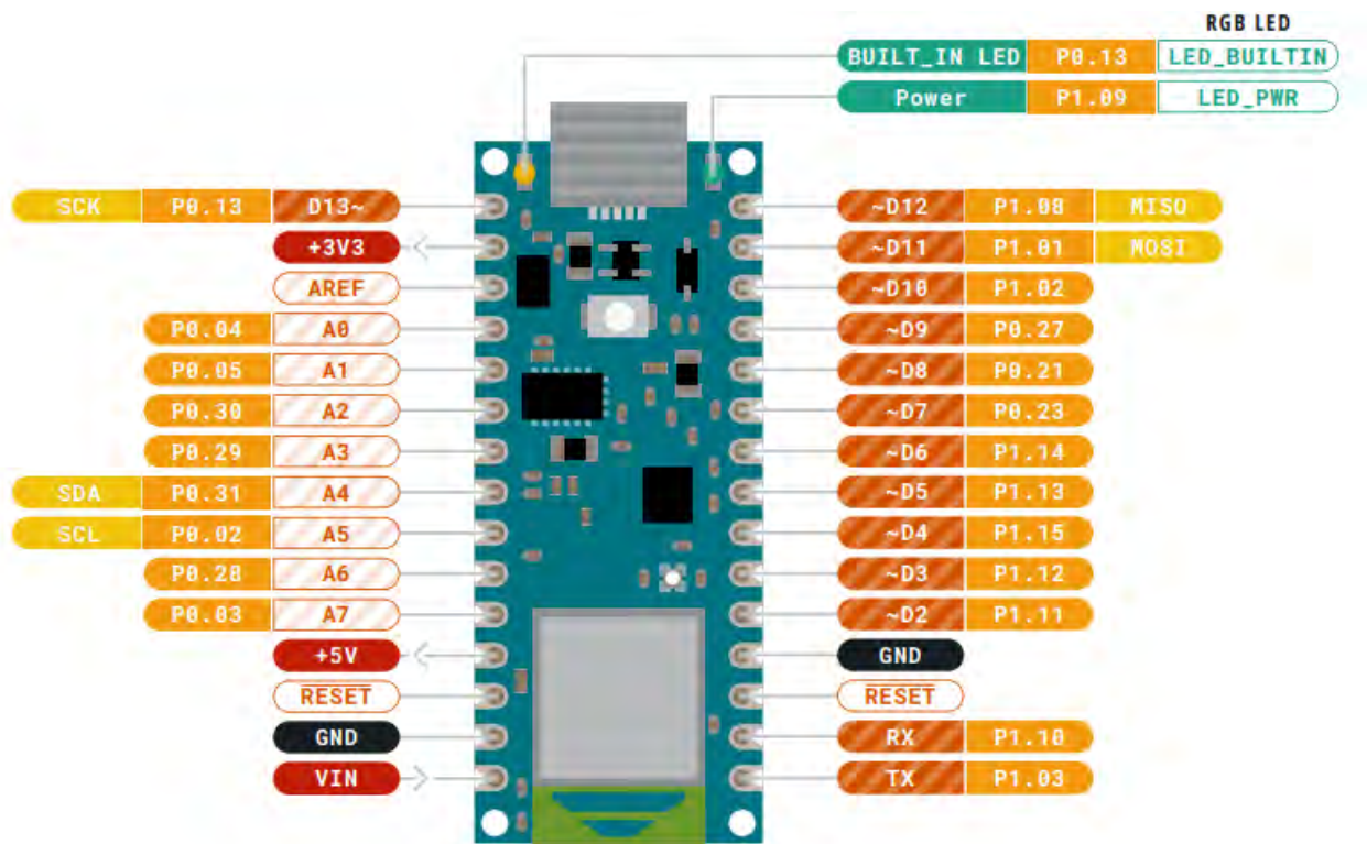
Pinout
