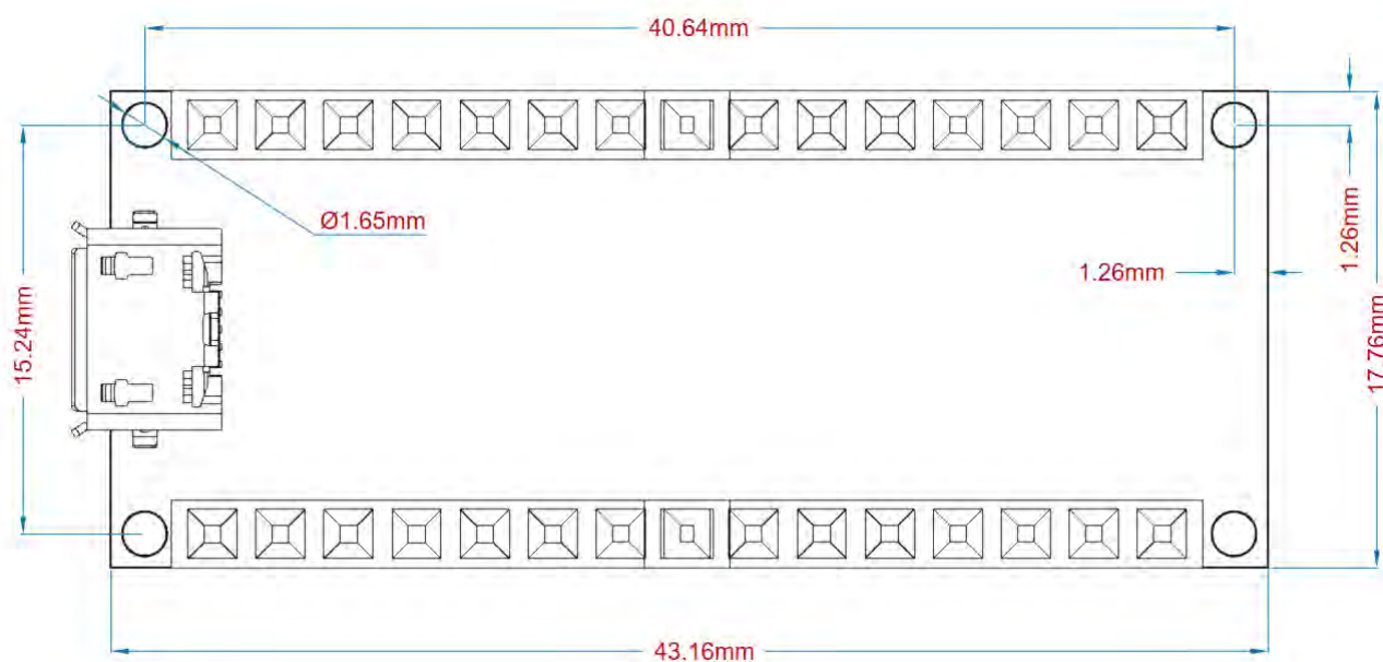
Board layout
