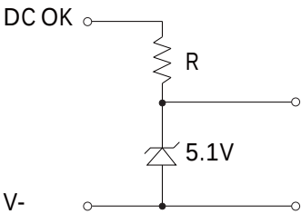
(a) 5V signal
